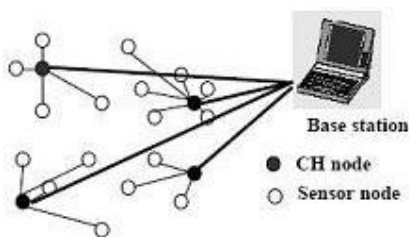
Figure 2. LEACH [7]
