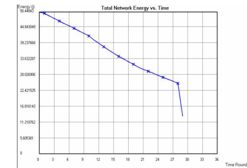
Figure 9. VGA total network energy
